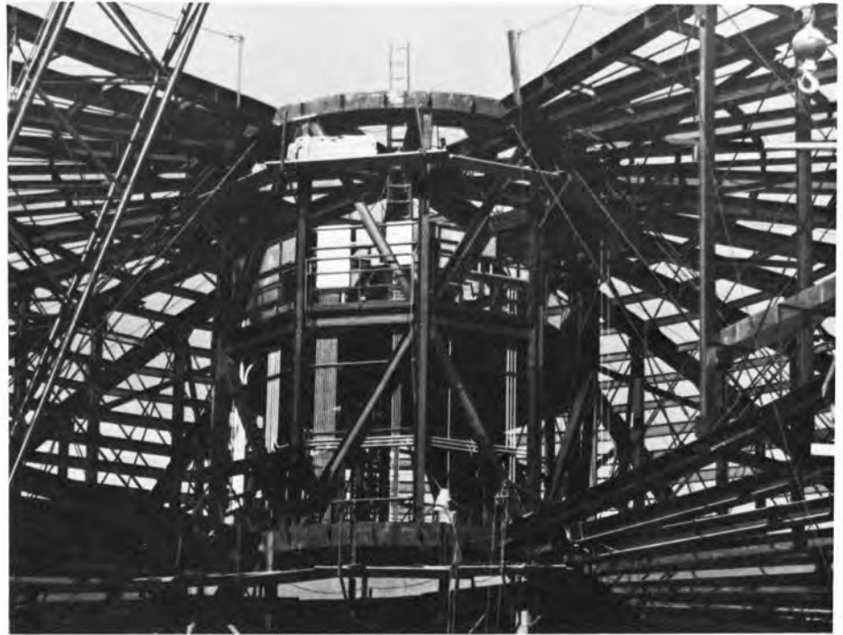
The frame of the scoreboard gets connected to the top.
